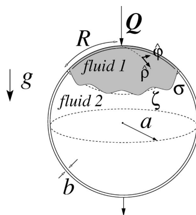
FIG. 1. Schematic configuration of flow in a spherical Hele-Shaw cell.
